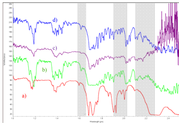
Figure 2: a) Pure acetonitrile at 89K b) Acetonitrile + ethane + tholins at 90K c) Pure ethane at 90K d) Ethane + tholins at 89K. Some of the visible tholins bands are shown in shaded region.
