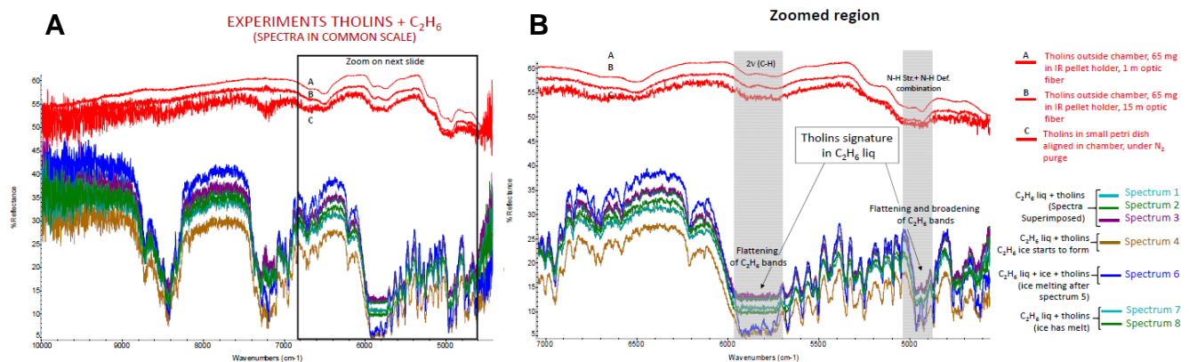
Figure 3: Spectra of tholins and ethane mixtures at 94 K (liquid \text{C}_2\text{H}_6 ) and 87 K (solid \text{C}_2\text{H}_6 ). The tholins were synthesized using our own plasma synthesis system, before being transferred into the Titan simulations chamber. A. Full spectral range allowed by the fiber optic (1 to 2.5 \mu\text{m} ). B. Zoom on the region where tholins signatures can be identified.
