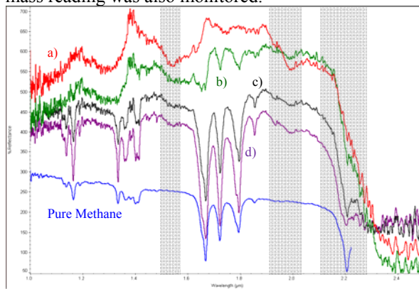
Figure 1: NASA AMES tholins in liquid methane. Some of the visible tholins bands are shown in shaded region. a) Tholins spectra at 1.5 bar and at 90 K. b) Methane + tholins spectra after evaporating methane at 138 – 149 K. c) Methane + tholins after couple hours into experiment at 89 K. d) Methane + tholins right after methane pour at 91 K.
